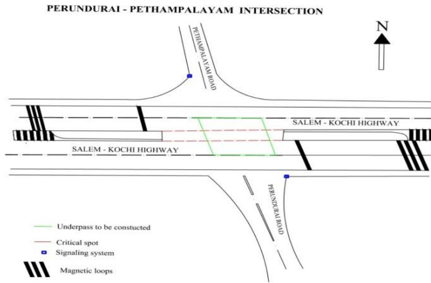
Fig 7. Safety measures provided in Perundururai – Pethampalayam intersection
