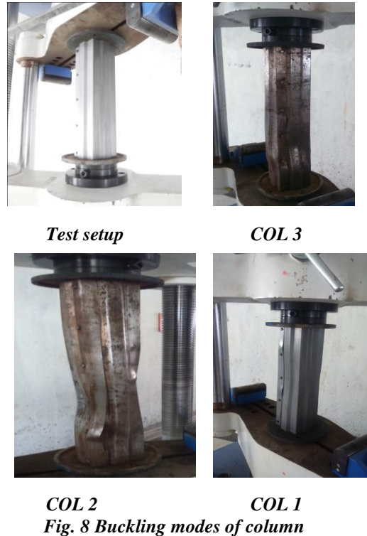
Fig. 8 Buckling modes of column
